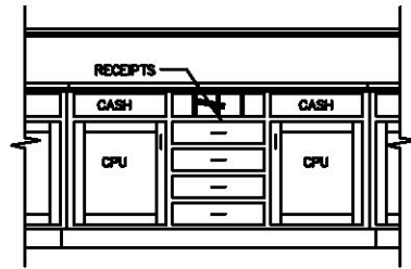
12 ELEVATION - 1/2" = 1'-0"
