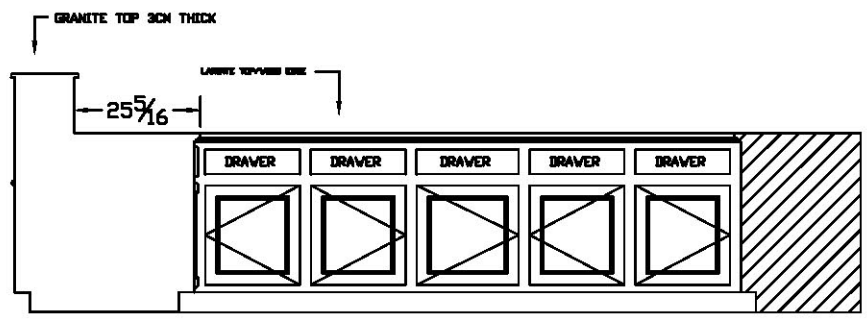
G ELEVATION 1/2" = 1'-0"
