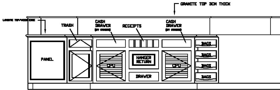
E ELEVATION 1/2" = 1'-0"
