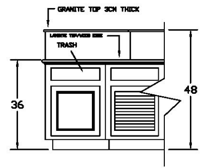
D ELEVATION 1/2" = 1'-0"
