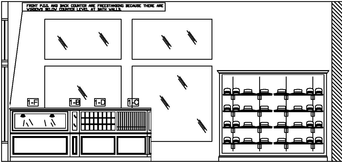
B ELEVATION 1/2" = 1'-0"
