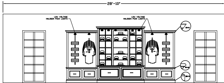
6 ELEVATION WOMEN'S DISPLAY AREA
