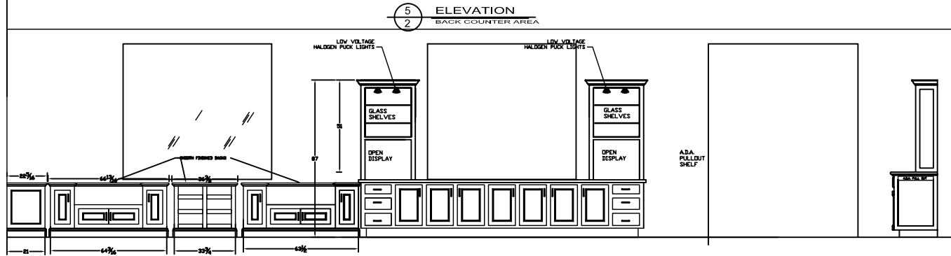
5 ELEVATION BACK COUNTER
