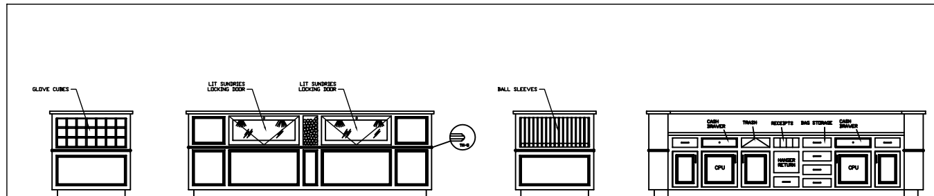
3 ELEVATION LEFT CUSTOMER SIDE
